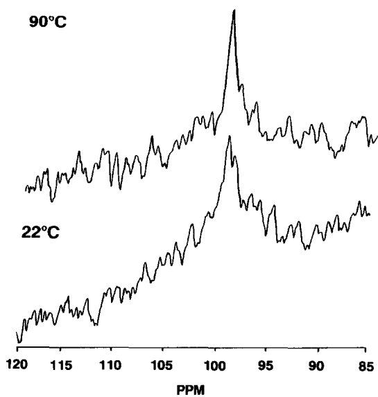
Figure 7 13 C spectral expansion of Figure 6, C 1 region
