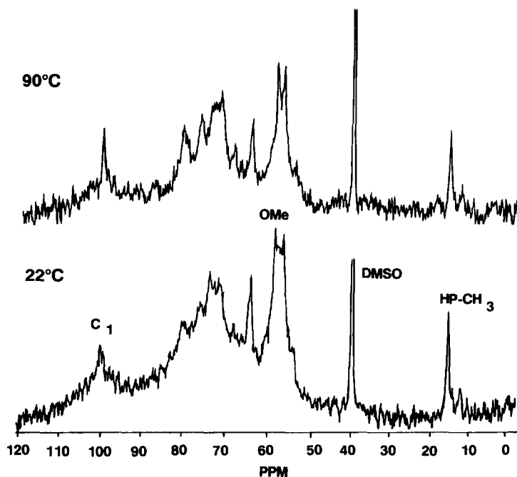
Figure 6 13 C spectra recorded at 90°C and 22°C of a 10% w/v solution of DP335 hydroxypropylmethylcellulose in D 2 O. Peak at 40 ppm is of the proteo-DMSO external standard in the coaxial capillary tube, which also contained 3 mg ml -1 Cr(AcAc) 3 relaxation reagent. The spectral intensities have been normalized to that of DMSO
