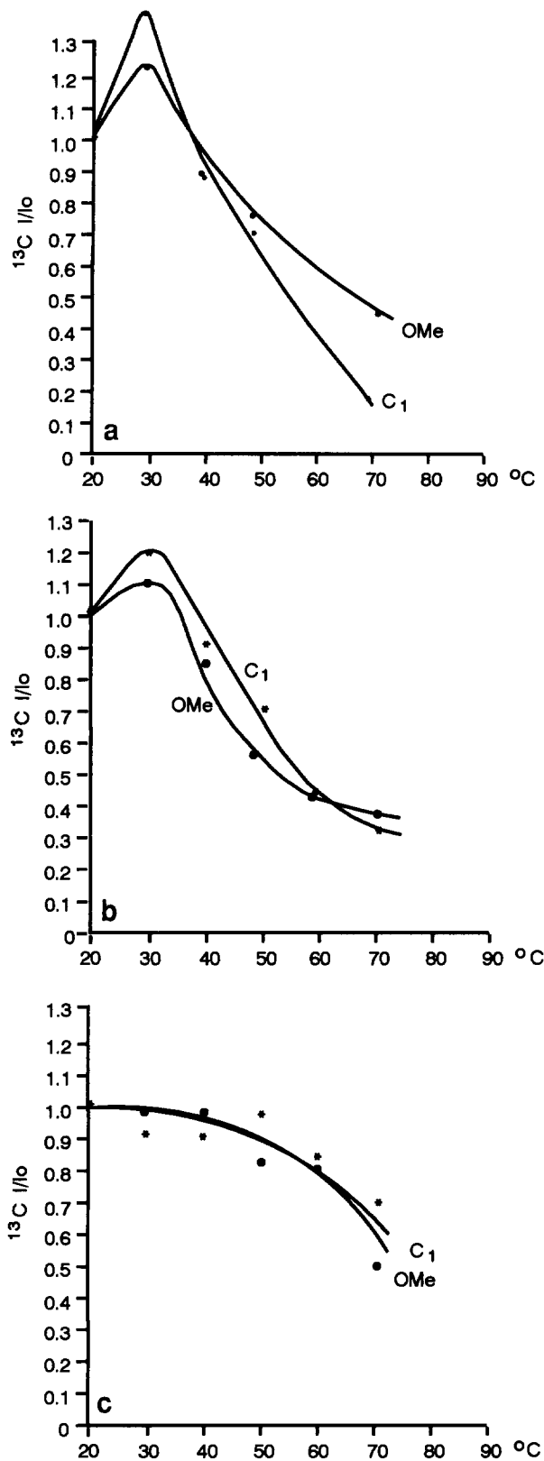
Figure 3 13 C intensities of C 1 and OMe signals of 10% w/v solutions of methylcellulose in D 2 O at different temperatures. In each case intensities were first normalized against that of an external DMSO standard normalized and then against the intensity of the signal at 22°C: (a) MM10; (b) M20; (c) MC90
