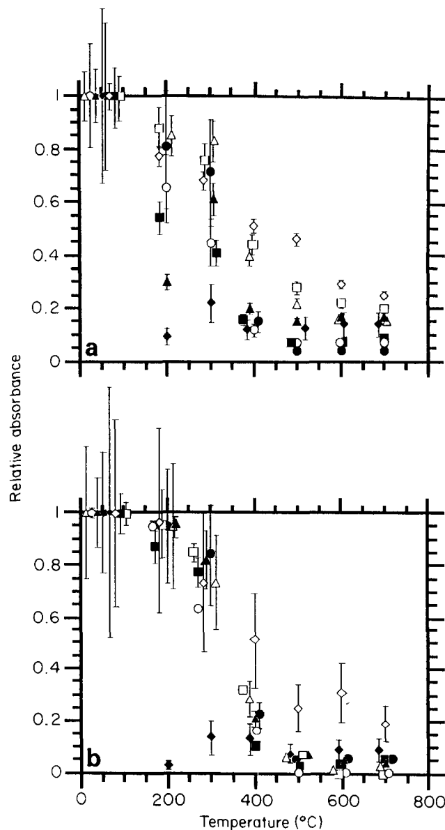
Figure 4 Relative absorbance at 350 nm of incorporated 2,4-dinitroaniline in sol-gel coatings as a function of temperature of thermal treatment (a) in air and (b) under argon. Samples were held at each temperature for 2 h. The relative absorbance is the ratio of the measured absorbance to that after an initial treatment at 100°C for 5 min. The symbols denote chromophore: (○) alone, (●) over porous SiO 2 , (△) with a dense SiO 2 overcoat, (▲) with a porous SiO 2 overcoat, (□) copolymerized in dense SiO 2 , (■) copolymerized in porous SiO 2 , (◇) physically mixed in dense SiO 2 , and (◆) physically mixed in porous SiO 2 . The points are shown displaced from the nominal temperatures to avoid overlap. The data points represent the average measurement of two samples, the error bars their range
